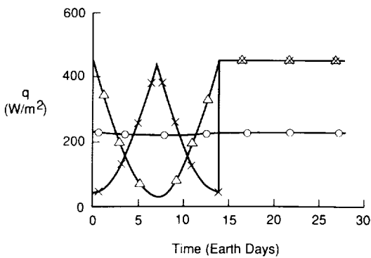
Fig. 7. (a) Heat rejection capability for radiators with a wall temperature of -6^{\circ}\text{C} at the South Pole. (b) Heat rejection capability for radiators with a wall temperature of 13^{\circ}\text{C} at the South Pole.
