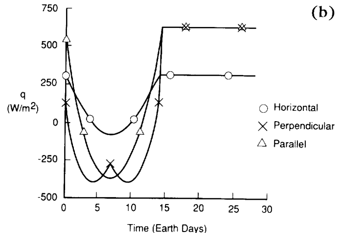
Fig. 8. (a) Heat rejection capability for radiators with a wall temperature of -6^{\circ}\text{C} at Lacus Veris. (b) Heat rejection capability for radiators with a wall temperature of 13^{\circ}\text{C} at Lacus Veris.
