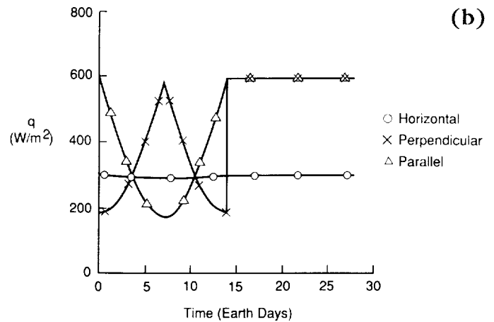
Fig. 7. (a) Heat rejection capability for radiators with a wall temperature of -6^{\circ}\text{C} at the South Pole. (b) Heat rejection capability for radiators with a wall temperature of 13^{\circ}\text{C} at the South Pole.
