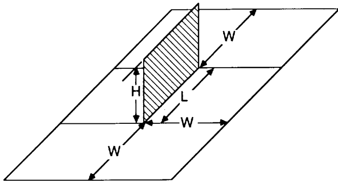
Fig. 9. Radiator and reflective insulation blanket model.
